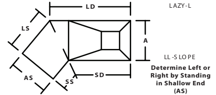
LAZY-L
